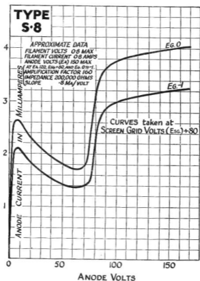
Characteristic Curve of Average S.8 Valve.
